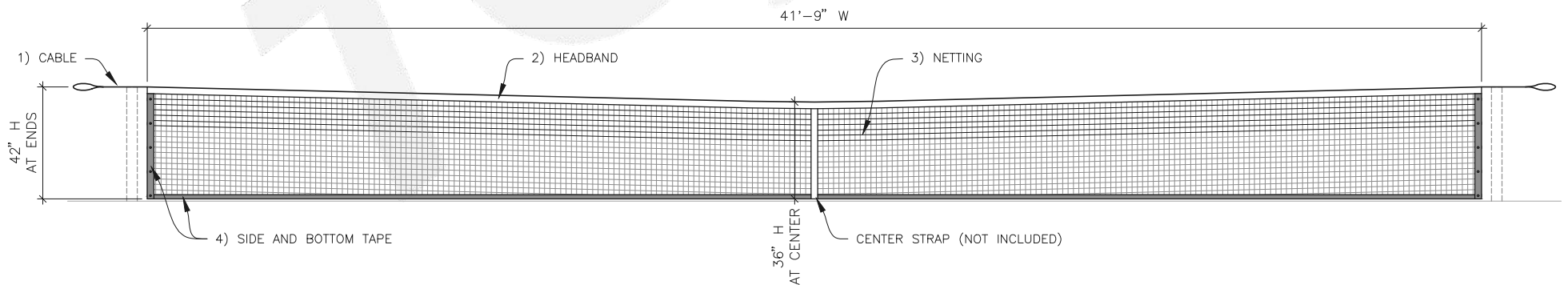
CHAMPIONSHIP TENNIS NET
